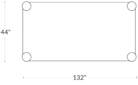
132" 10-12 SEATS 132" L x 44" W x 30" H
